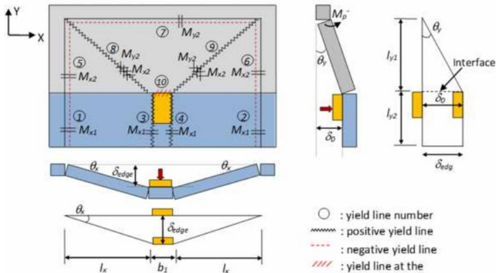
Fig 3. The assumed yield line mechanism for the PC deck slabs with interface.
