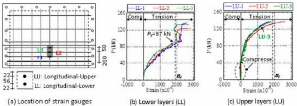
Fig 9. Strain in the longitudinal rebars (SL-P1.0).
