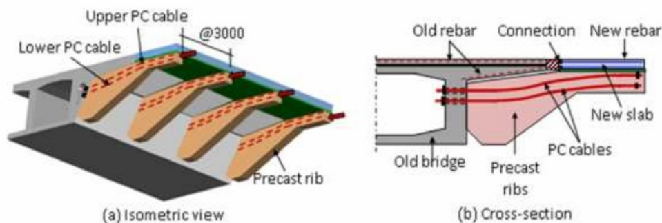
Fig 1. The new prestressed concrete (PC) box girder widening technique.
