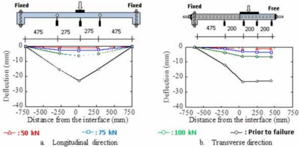
Fig 8. Deflection distributions of SL-P1.0.
