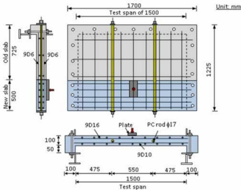
Fig 4. Deck slab layout and reinforcement details.
