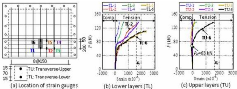
Fig 10. Strain in the transverse rebars (SL-P1.0).
