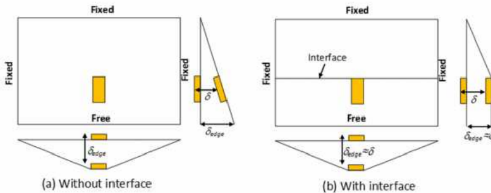
Fig 2. Influence of the interface on the deflection distributions.
