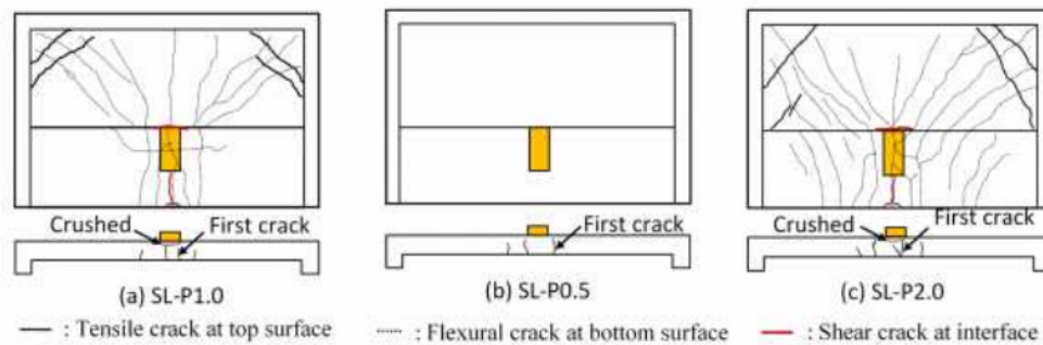
Fig 7. Experimental crack patterns.
