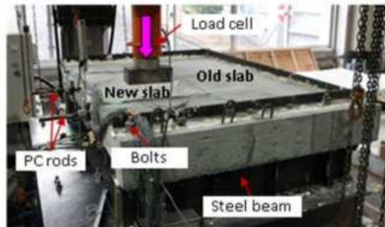
Fig 5. Photograph of the test.
