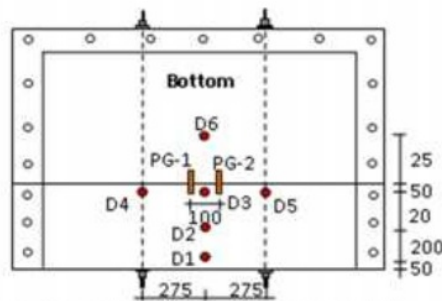
(a) Location of transducers and \pi -gauges
